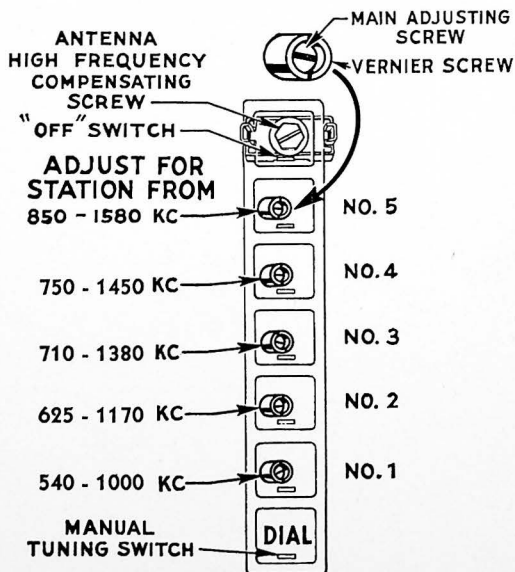
AUTOMATIC ADJUSTING SCREWS
